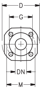
PUMP FLANGES
